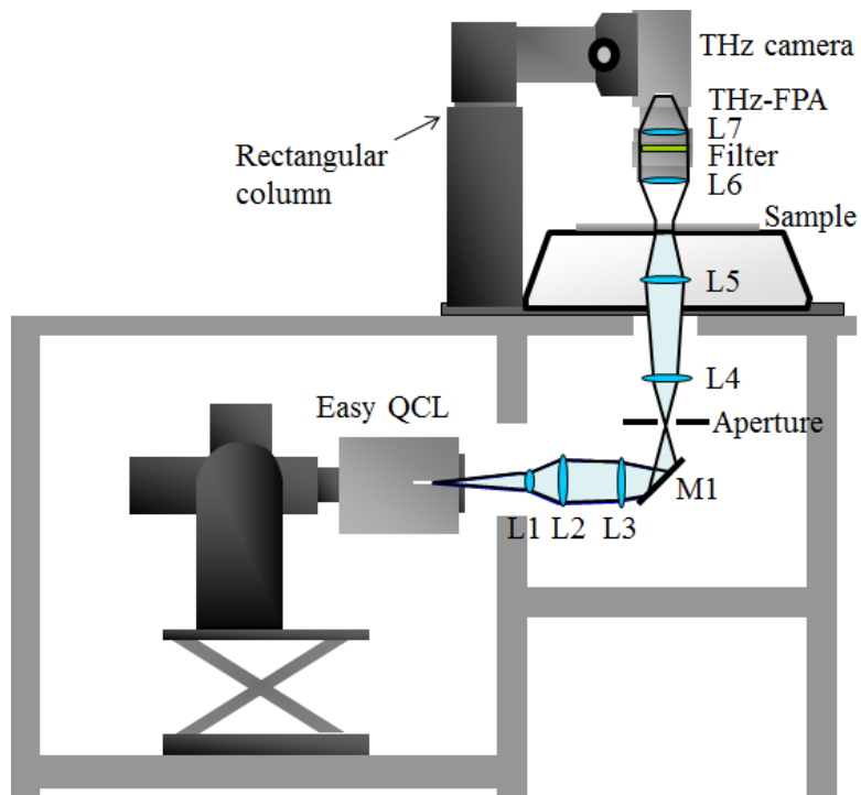
Fig.2 A layout of transmission-type THz microscope
