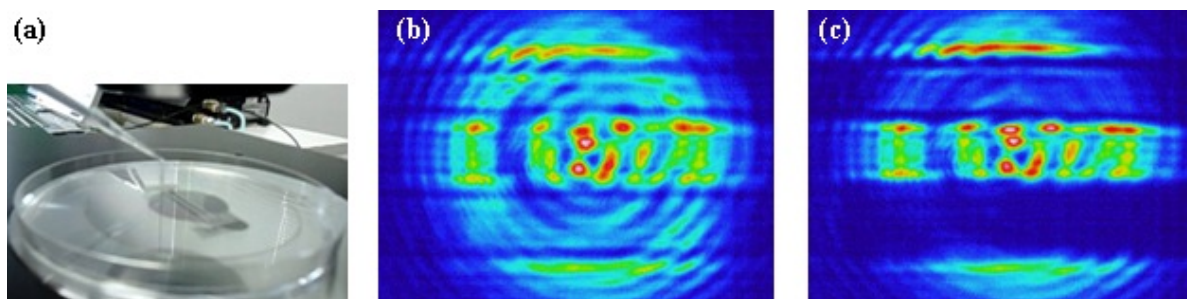
Fig.10 (a) Sample setup, (b) THz image prior to flowing ethanol and water, (c) THz image during flowing ethanol (upper) and water (lower).
