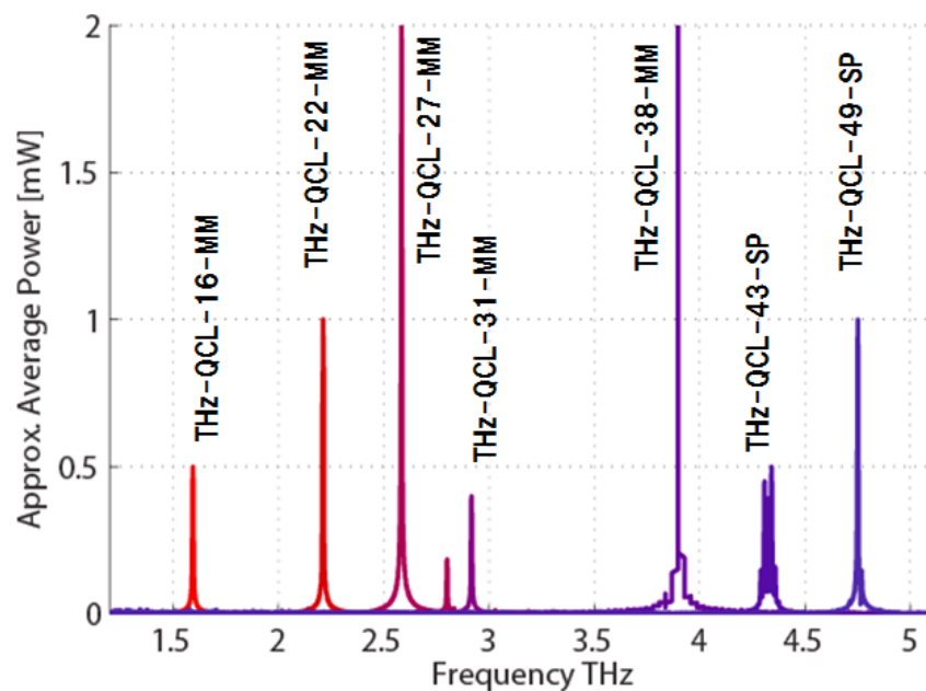
Fig.5 Frequency dependence of approximate time-average powers from QCLs (operation temperature: ca. 50 K)
