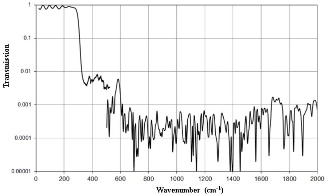
Fig.3 Transmission curve of the infrared blocking filter (QMC Instruments, Ltd)
