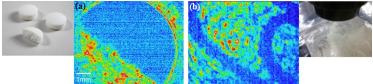
Fig.9 (a) Visible picture of tablet (left) and THz image of tablet put inside envelope (right) [frame integration: 2, spatial filter: 4x4] and (b) THz image of metallic clip put under flours (left) and visible picture of sample (right) [frame integration: 4, spatial filter: 2x2]. Both images were taken with lock-in imaging function (lock-in frequency 3.75 Hz).
