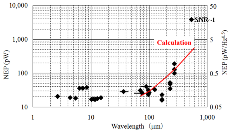
Fig.7 Wavelength dependence of NEP for THz-FPA itself (Data point at 550 \mu\text{m} has SNR of ca. 1)
