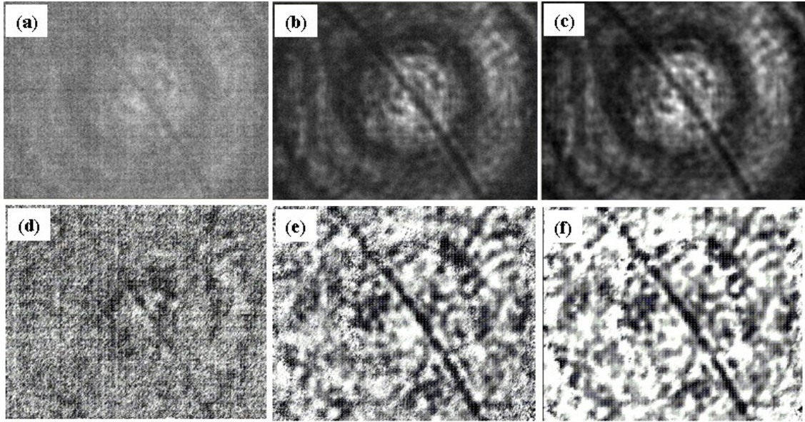
Fig.8 THz images of human hair put under a sheet of paper. (a) Real-time image (no lock-in function, no frame integration, no spatial filter : SNR~3.4), (b) Lock-in image (lock-in frequency 3.75Hz, 16 frames integration, no spatial filter : SNR~16), (c) Lock-in image (lock-in frequency 3.75Hz, 16 frames integration, 3x3 spatial filter : SNR~47). Images shown in (d), (e) and (f) were obtained with the procedure described in the text.
