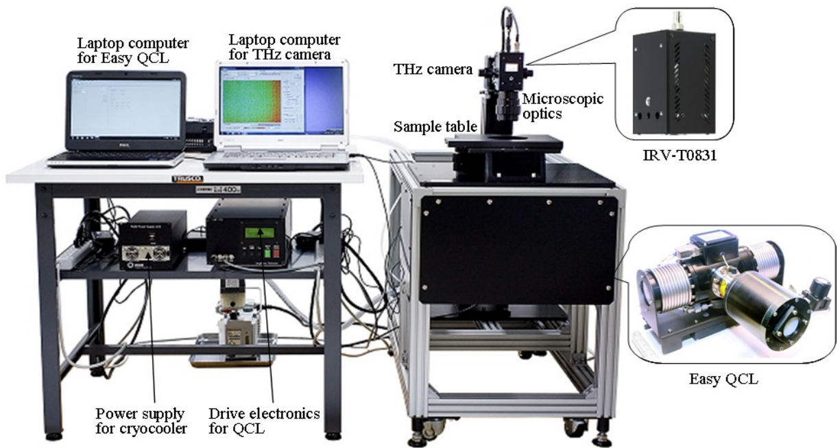
Fig.1 A picture of transmission-type THz microscope
