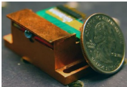
Fig.4 Packaged QCL with hyper-hemispherical lens
